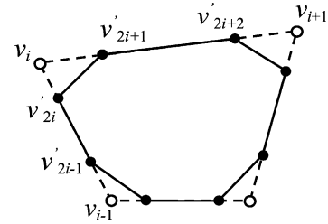
Fig. 2. Topological rules for Chinkin’s subdivision.
